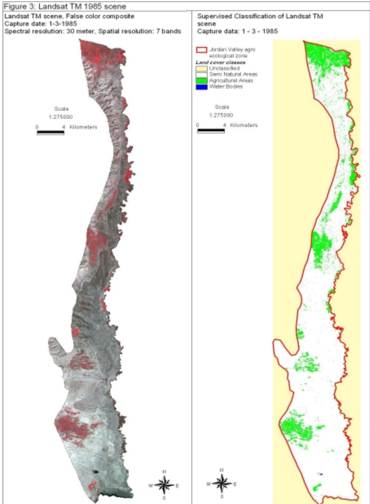
Fig. 3. Shows landsat TM scene on the left side and the derived thematic data of the supervised classification on the right side.
